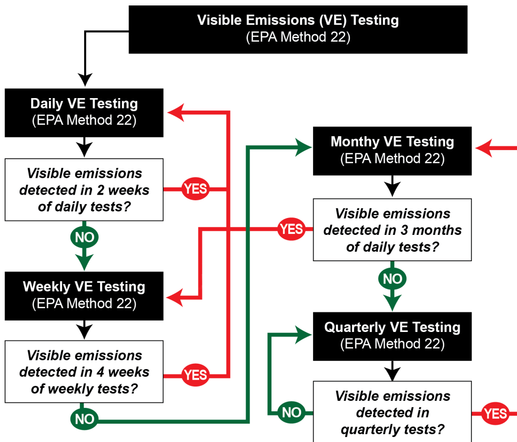
Figure 1: Visual Determination of Fugitive Emissions
